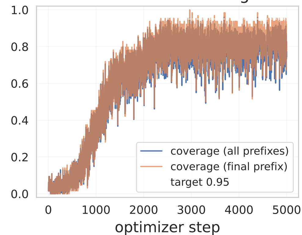
Gaussian x-likelihood noise
