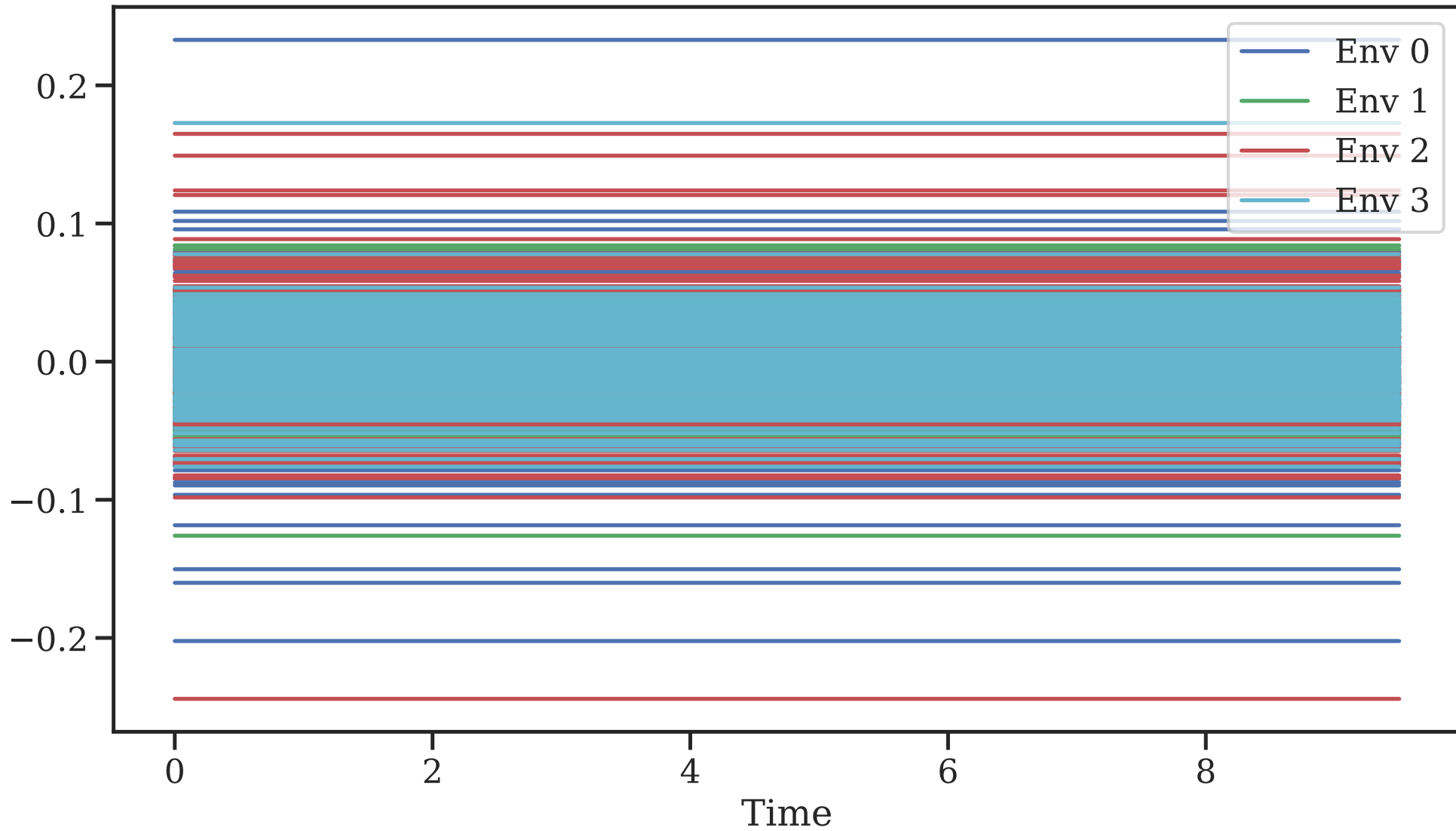
Context Predictions
