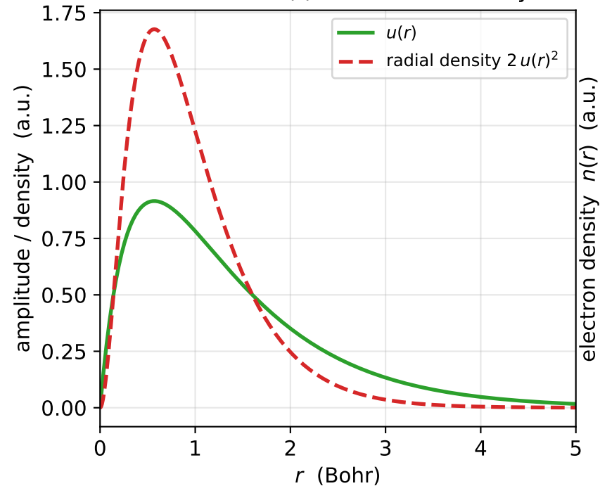
M5 orbital u(r) and radial density
