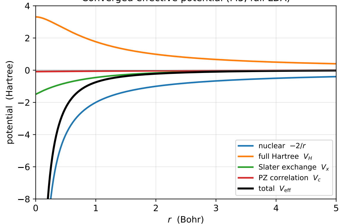
Converged effective potential (M5, full LDA)
