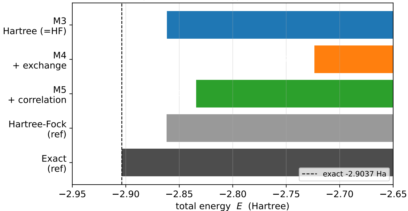
Helium ground-state energy: this work vs references
