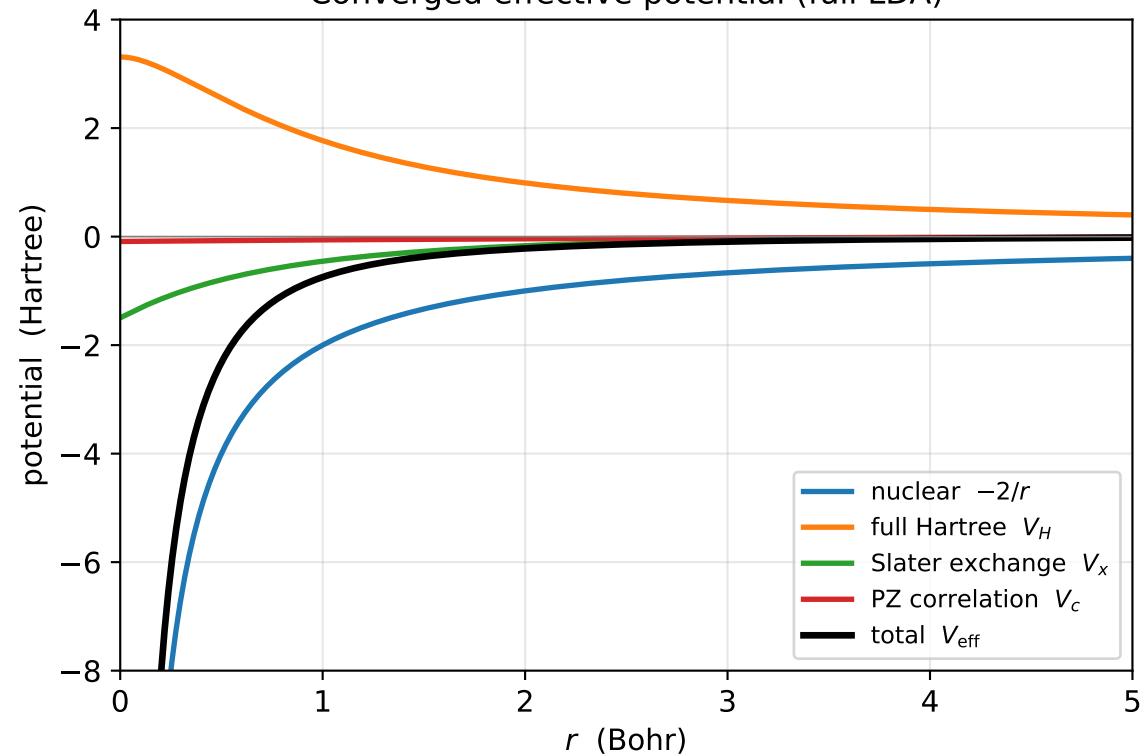
Converged effective potential (full LDA)
