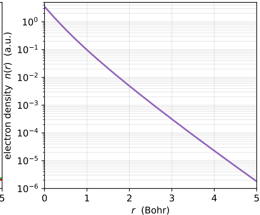
Full density n(r) = u^2/(2\pi r^2)
