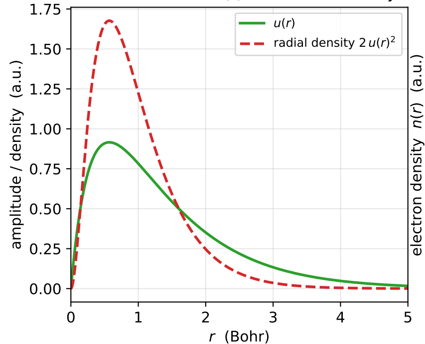
Full-LDA orbital u(r) and radial density
