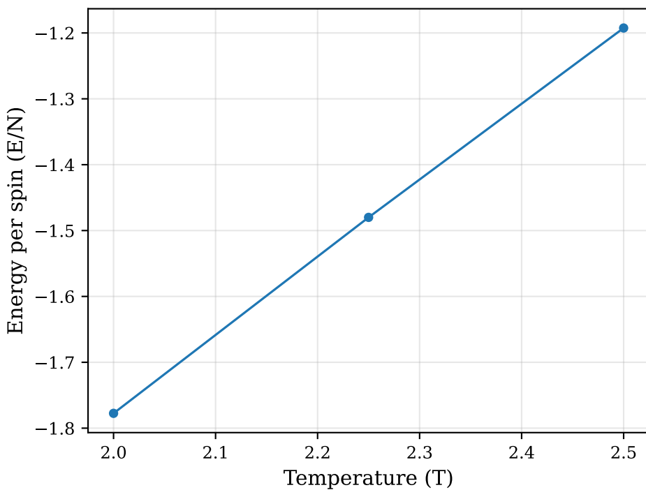
Phase Diagram (L=8)
