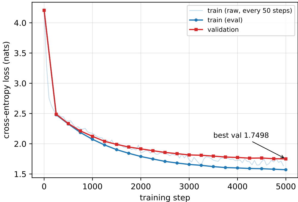
Picoder 0.1: training and validation loss
