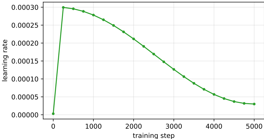
Picoder 0.1: learning-rate schedule (warmup + cosine decay)
