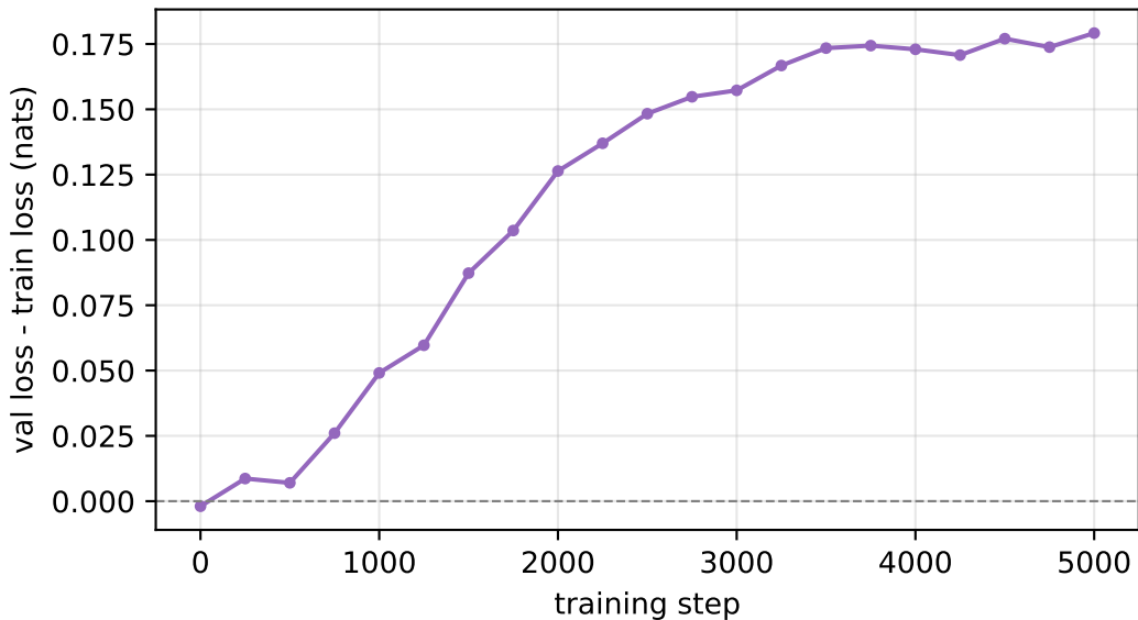
Picoder 0.1: generalization gap
