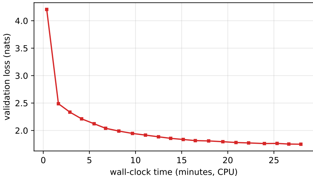
Picoder 0.1: validation loss vs wall-clock time
