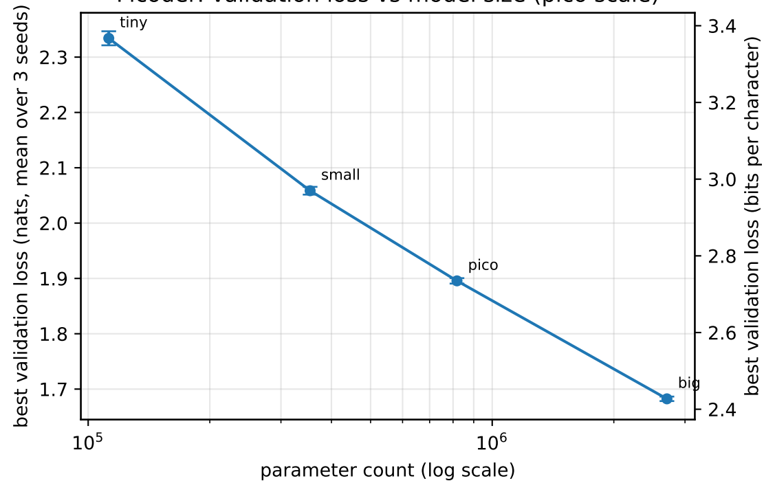
Picoder: validation loss vs model size (pico scale)
