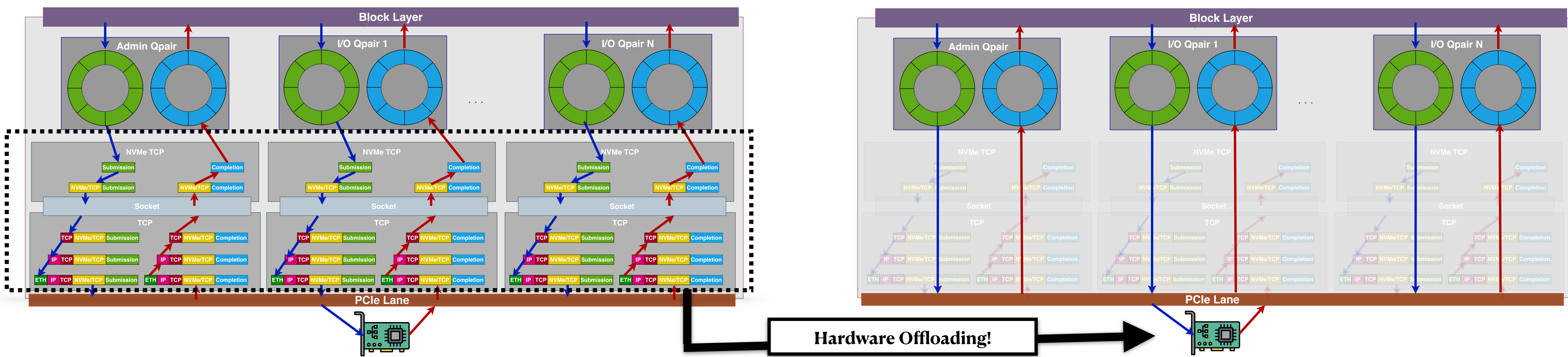
Existing system with CPU-processed TCP and NVMe/TCP
