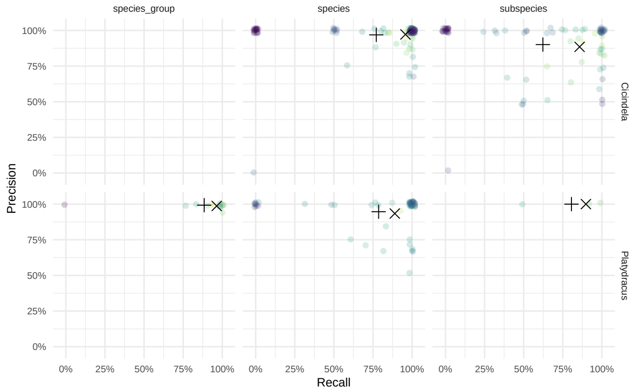
C Precision and Recall
