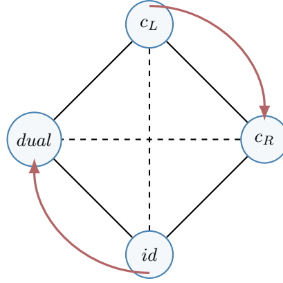
Figure 15.1: Automorphism action on the four-case witness space: preserve and swap survive as the only orbit structure.
