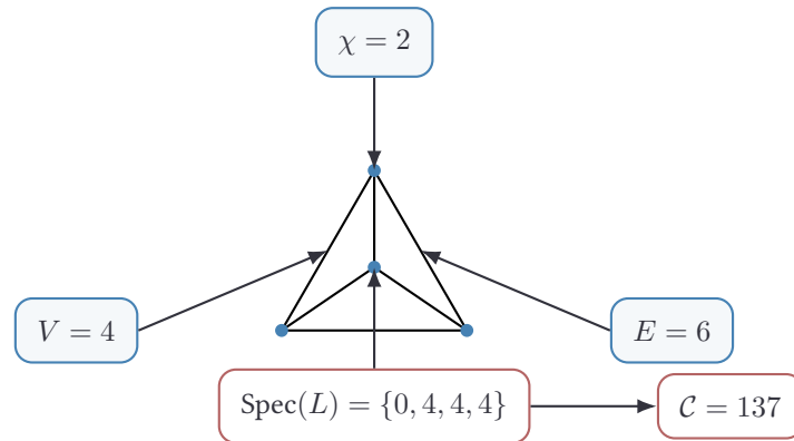
Figure 29.1: The basic combinatorial and spectral data of K_4 assembled into the invariant ledger.
