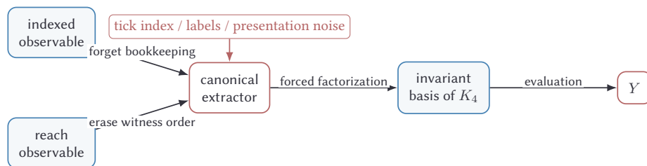
Figure 27.1: Admissible observables factor through the canonical invariant basis once presentation-dependent bookkeeping has been removed.
