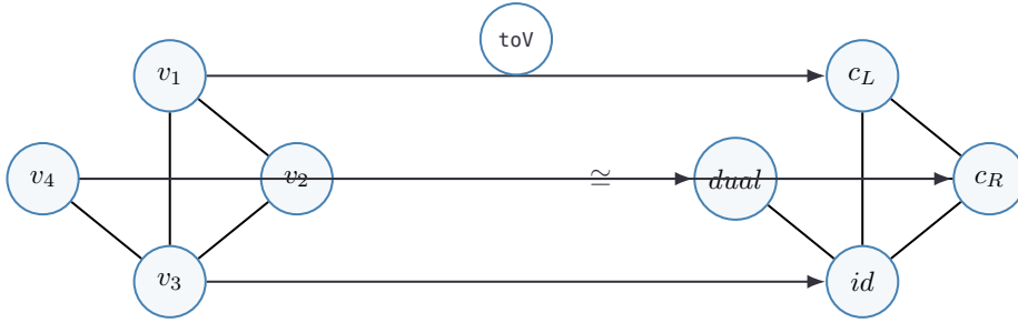
Figure 28.1: Any four-vertex presentation of the endomorphism classes collapses, by relabelling, to the canonical graph on EndoCase.
