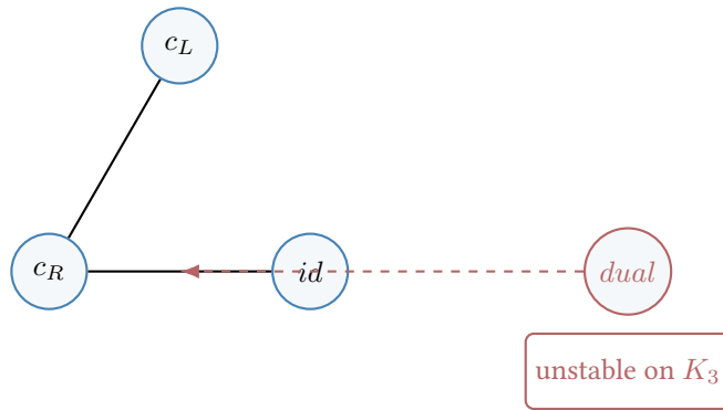
Figure 14.2: The failure of K_3 : the four mathematically distinct endomorphism cases cannot close over three vertices. One function is structurally forced into non-closure.
