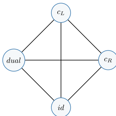
Figure 14.3: Exhaustive four-case endomorphism classification closes as the complete graph K_4 .
