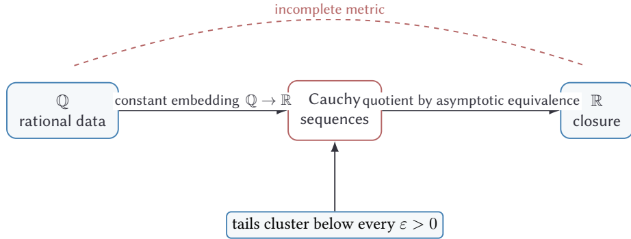
Figure 55.1: Forced Cauchy closure: \mathbb{Q} embeds as constant sequences, while the missing limits of rational Cauchy data are closed inside \mathbb{R} .
