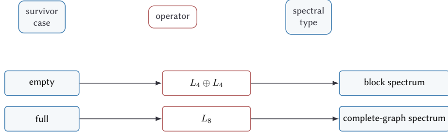
Figure 47.1: Coupling survivor dispatch. Empty and full are the two constructors of the survivor type, and each determines one operator and one spectral regime.
