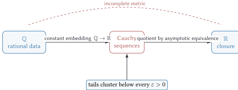
Figure 52.1: Forced Cauchy closure: \mathbb{Q} embeds as constant sequences, while the missing limits of rational Cauchy data are closed inside \mathbb{R} .
