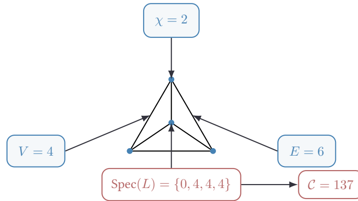
Figure 26.1: The basic combinatorial and spectral data of K_4 assembled into the invariant ledger.
