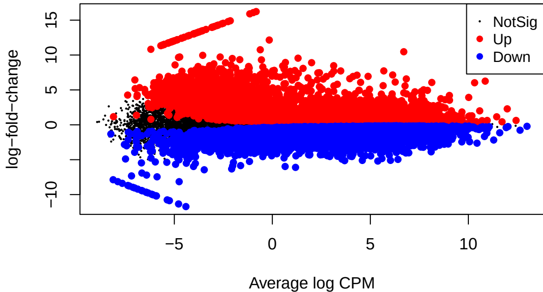
MA plot for DEG's
