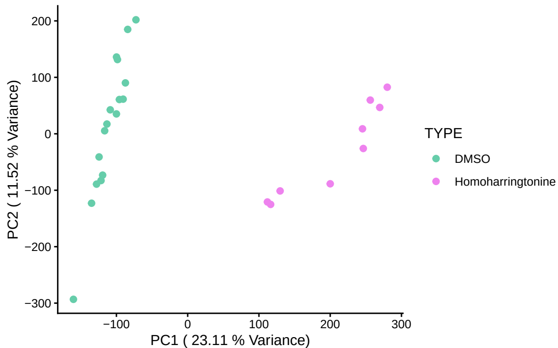
PCA after outlier removal
