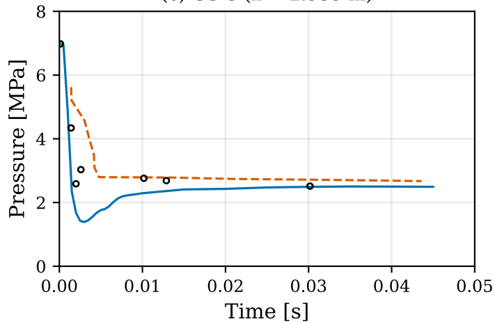
(c) GS-3 ( x = 2.935 m)
