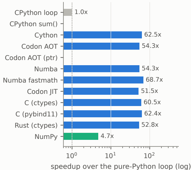
mandelbrot 200x150
