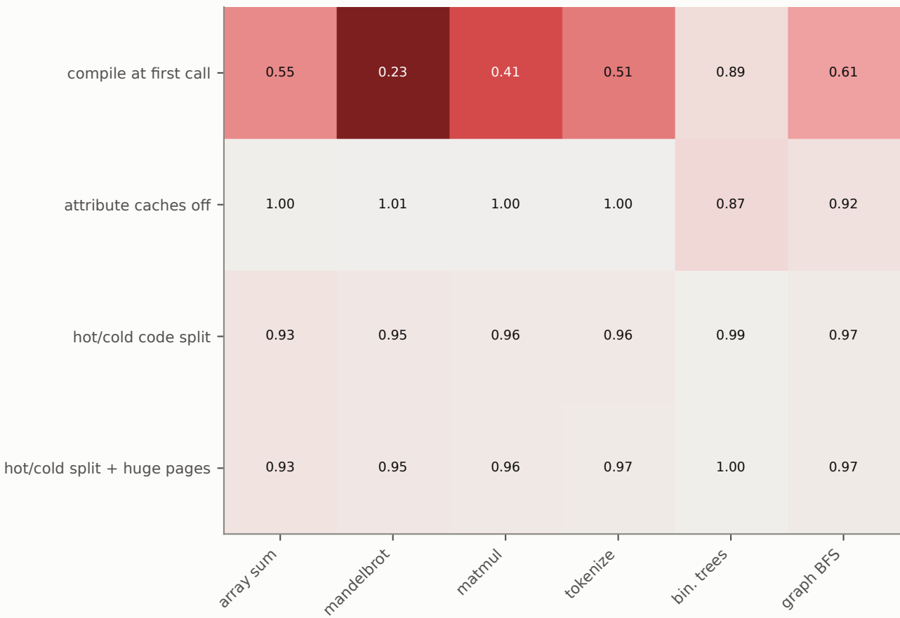
Speed relative to the default JIT configuration (&gt;1 = faster)
