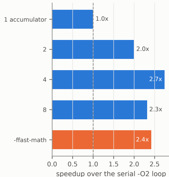
Regrouped in the source, at -O2
