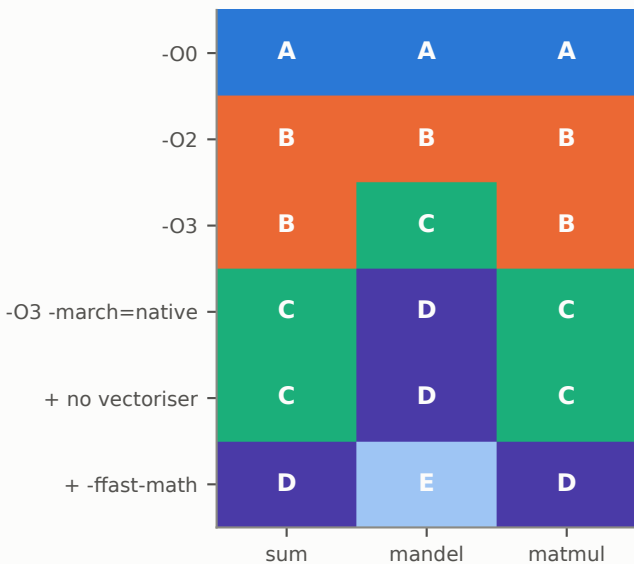
Same letter = same machine code
