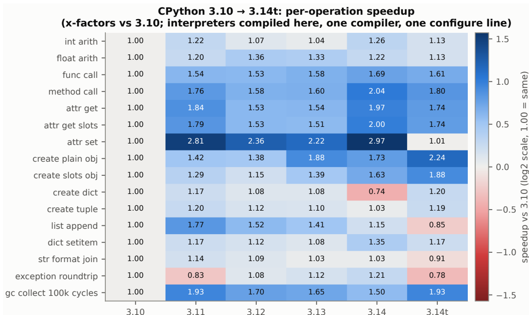
Figure 6: RQ3: per-operation speedup relative to CPython 3.10 (values are \times factors; blue = faster, red = slower).
