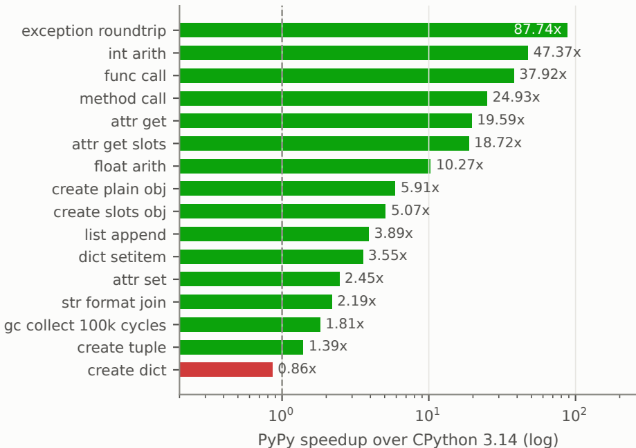
Interpreter-level operations
