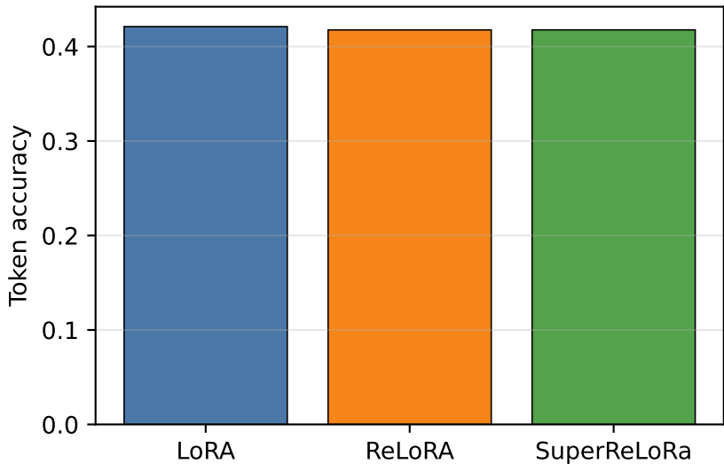
Token accuracy
