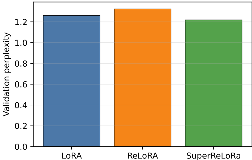
Validation perplexity
