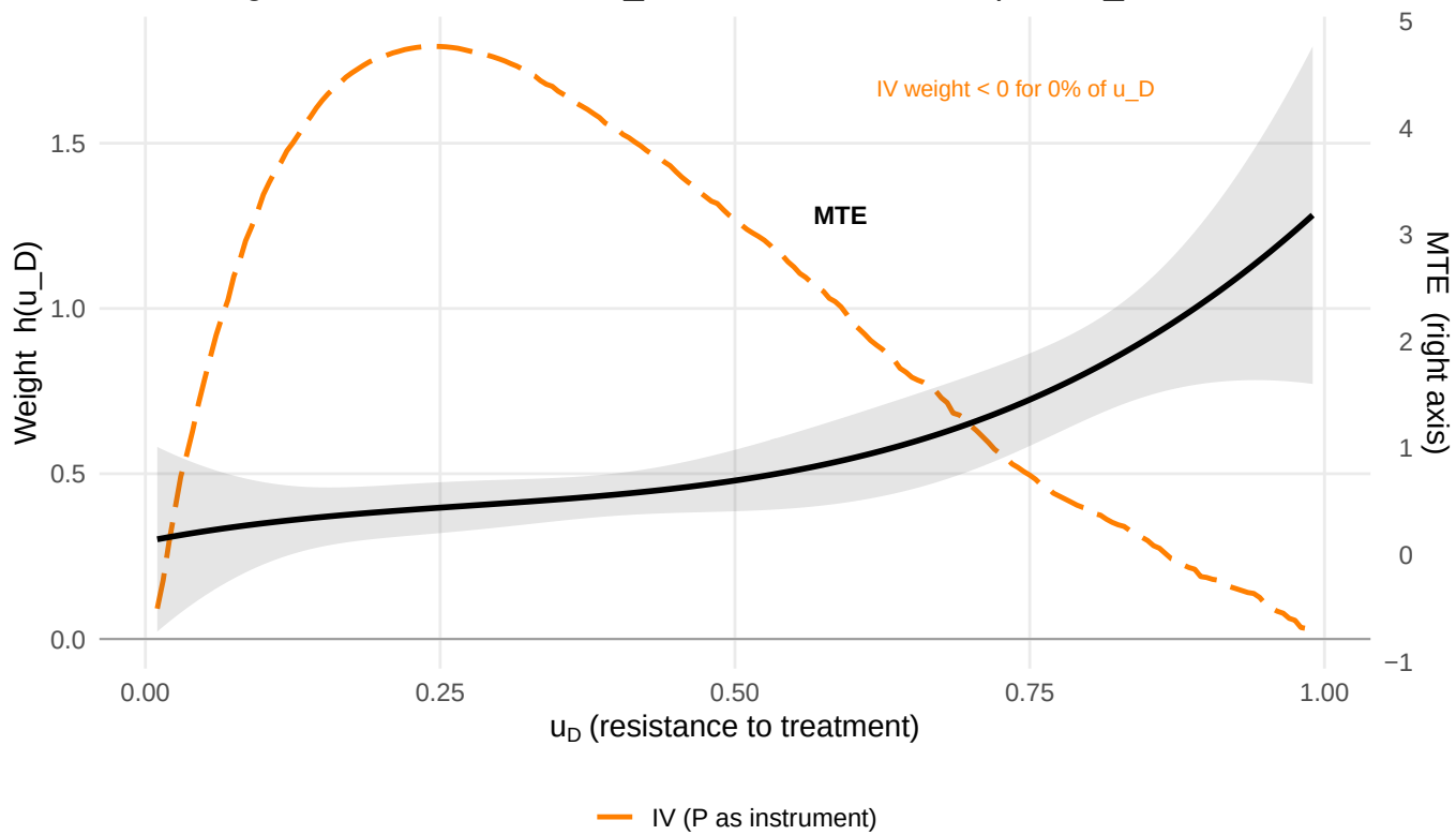
MTE Weights — outcome: fascist_branch, instrument: exposure_stat
