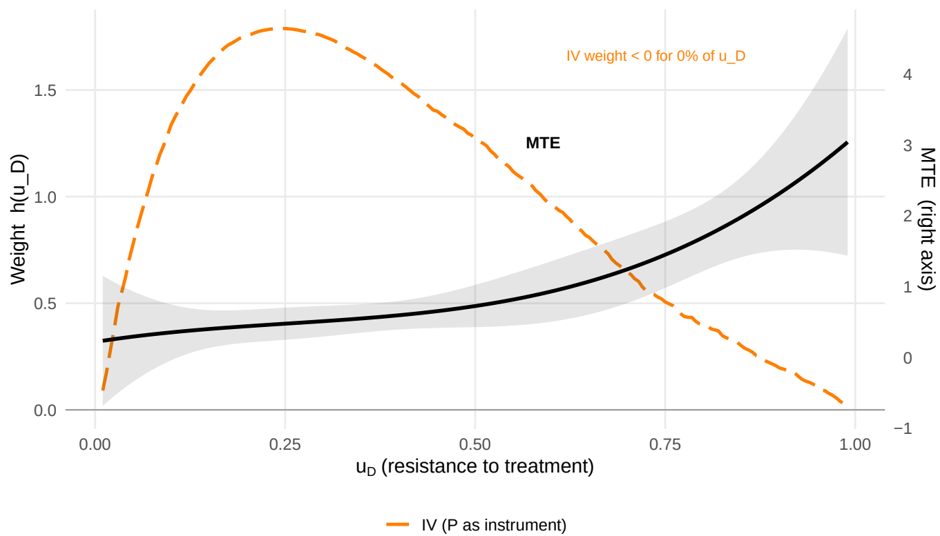
MTE Weights — outcome: fascist_branch, instrument: stat
