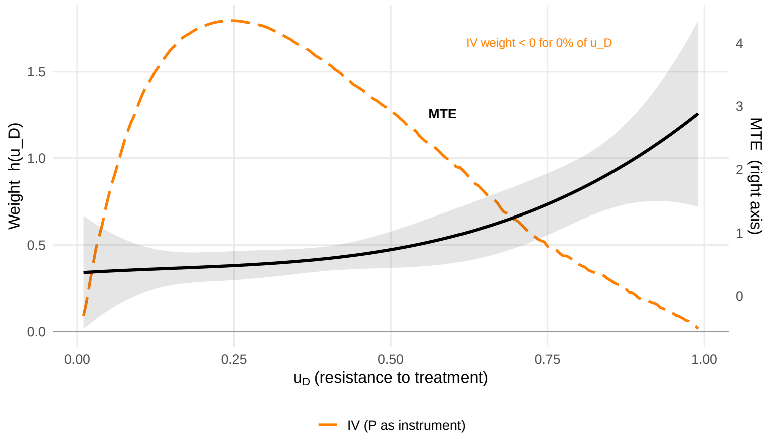
MTE Weights — outcome: fascist_branch, instrument: stat + Monte
