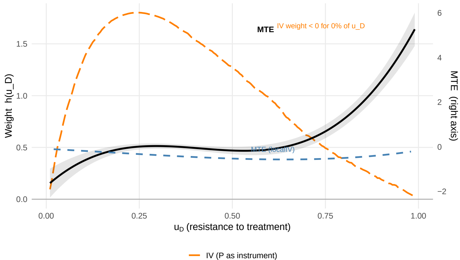
MTE Weights — outcome: dlf_1926, instrument: Monte
