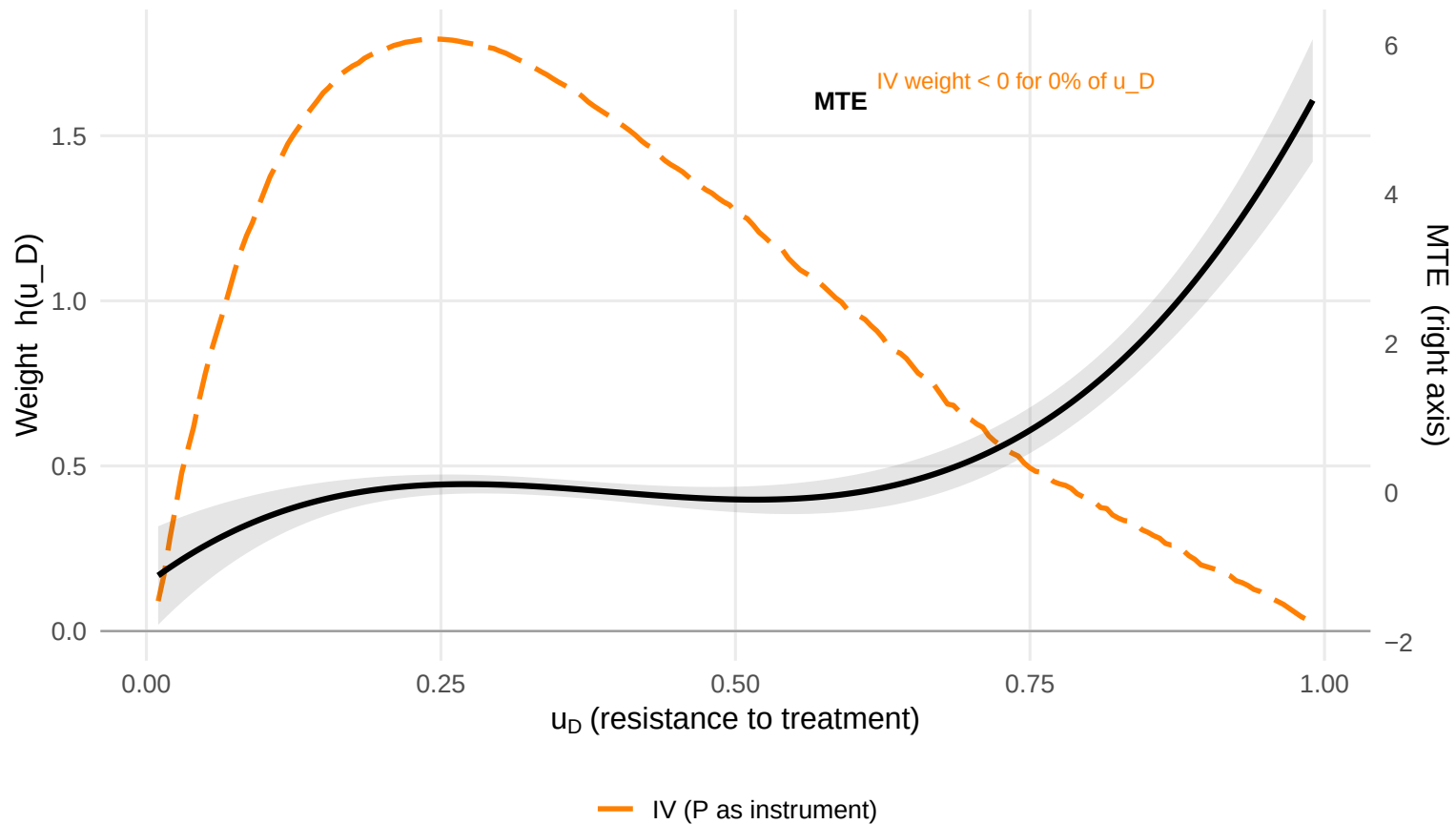
MTE Weights — outcome: dlf_1926, instrument: stat
