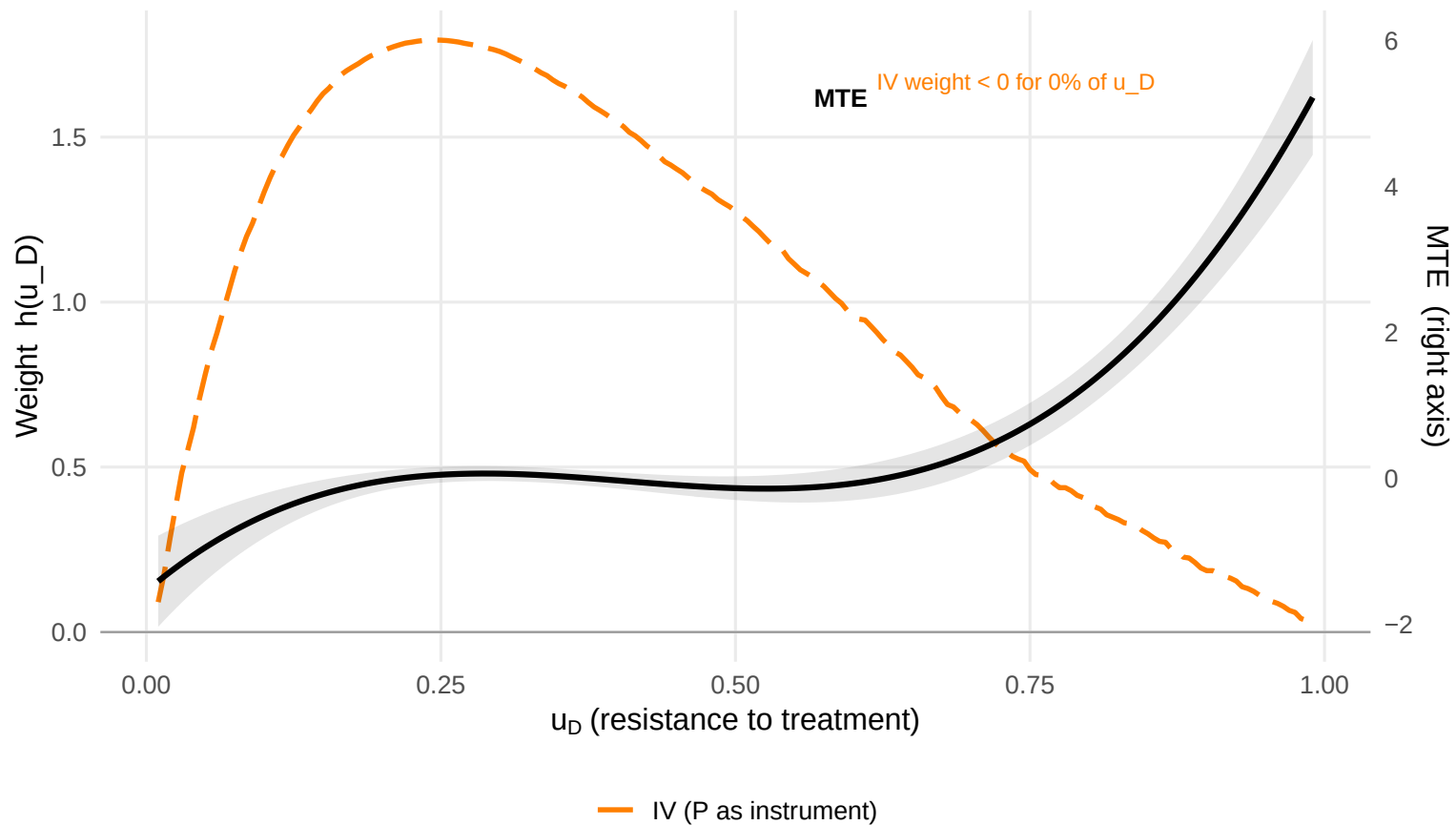
MTE Weights — outcome: dlf_1926, instrument: stat + Monte
