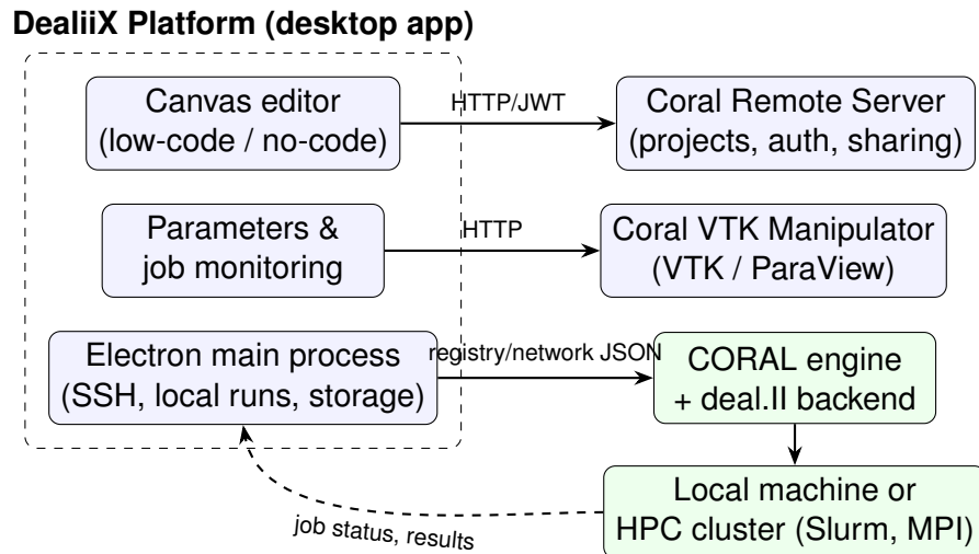
Figure 1: Architecture of the PoC platform and its components
