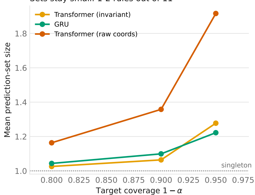
Sets stay small: 1-2 rules out of 11
