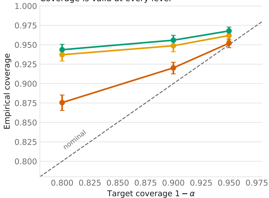
Coverage is valid at every level
