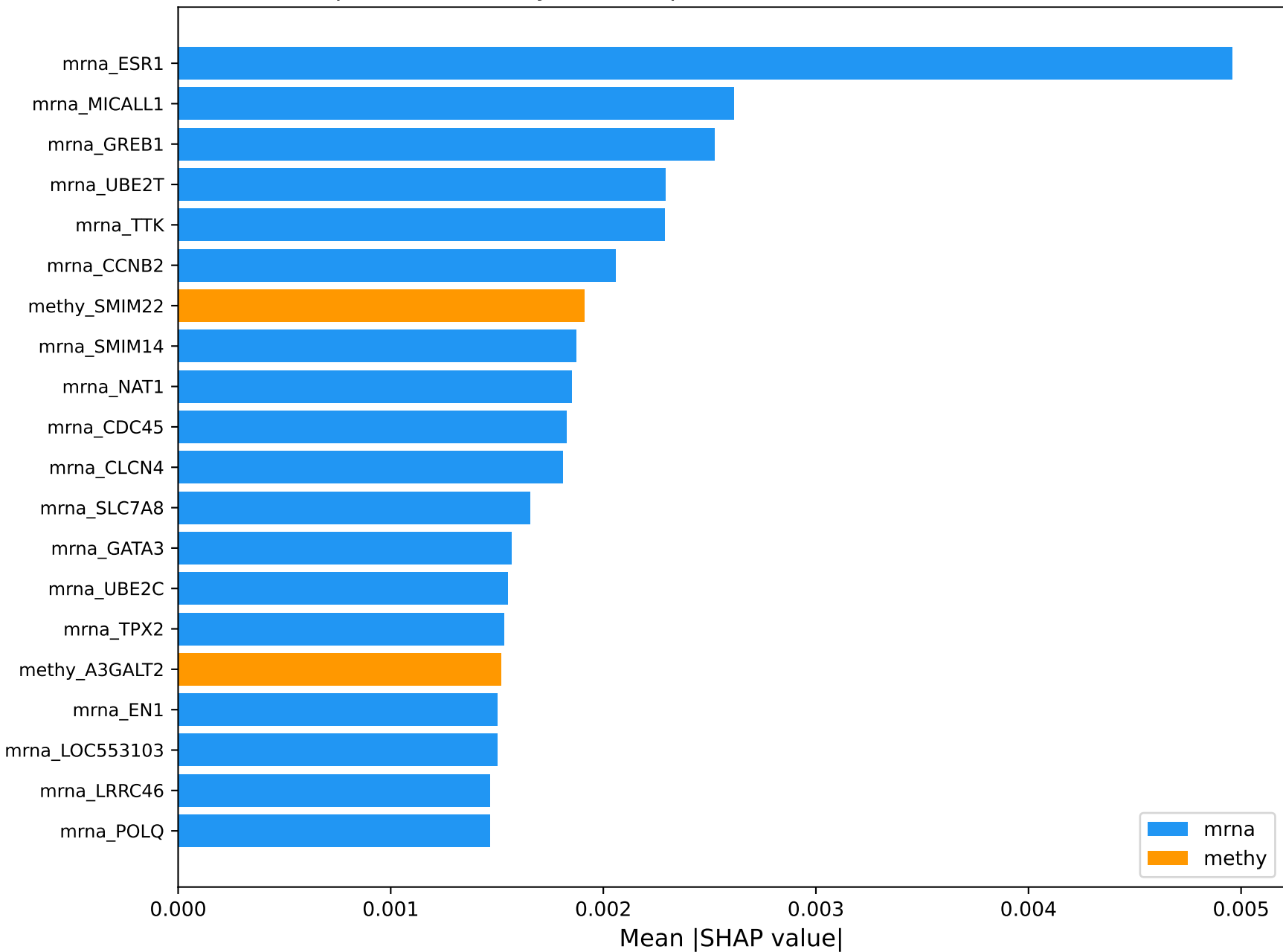
Top 20 Features by SHAP Importance — RandomForest (GS-BRCA)
