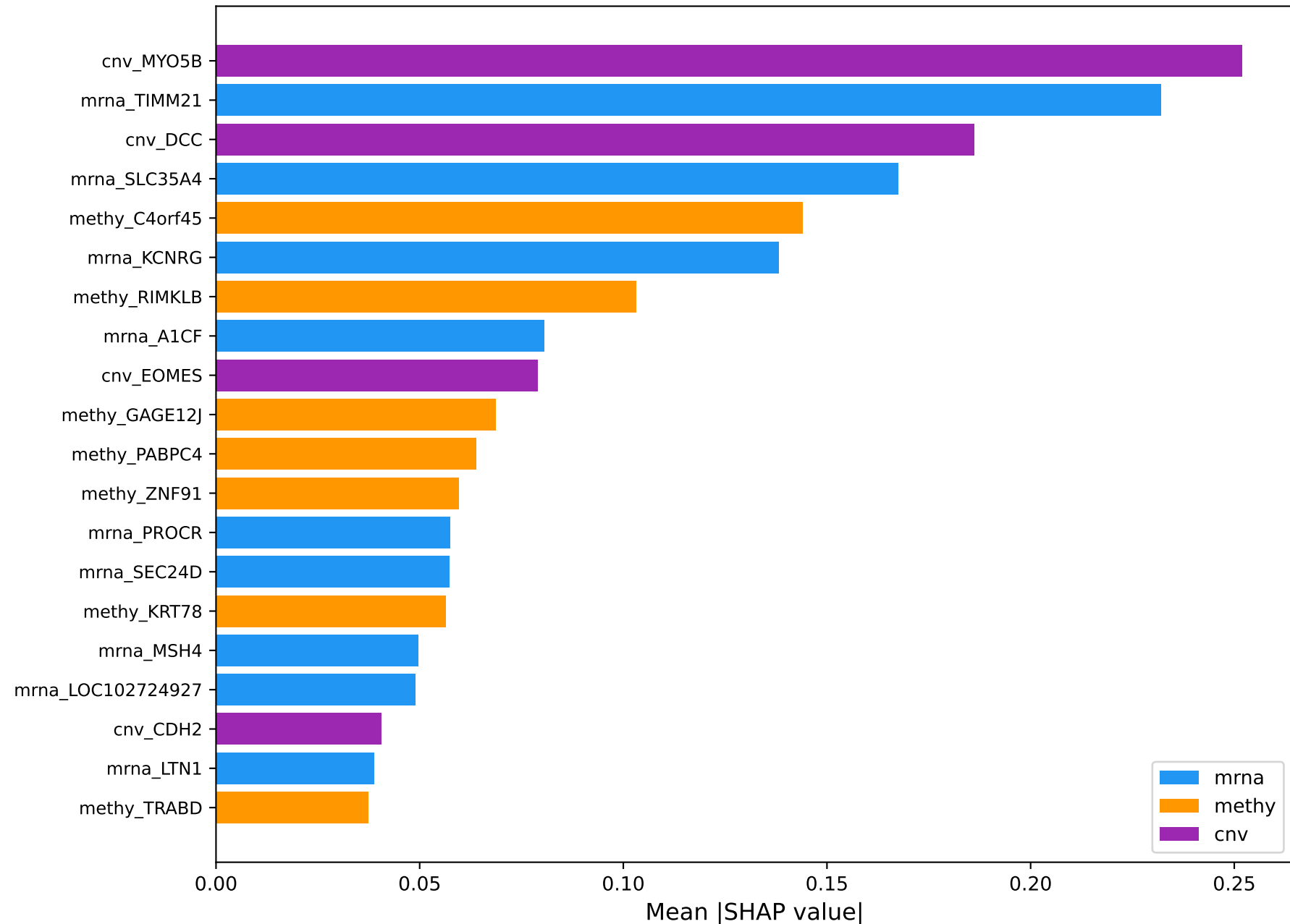
Top 20 Features by SHAP Importance — XGBoost (GS-COAD)
