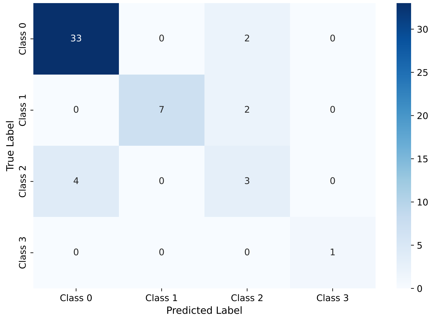
Confusion Matrix: IntermediateFusion (GS-COAD) Best Fold 3 (F1=0.8051)
