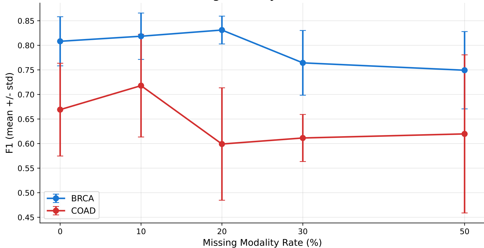
Missing Modality Robustness
