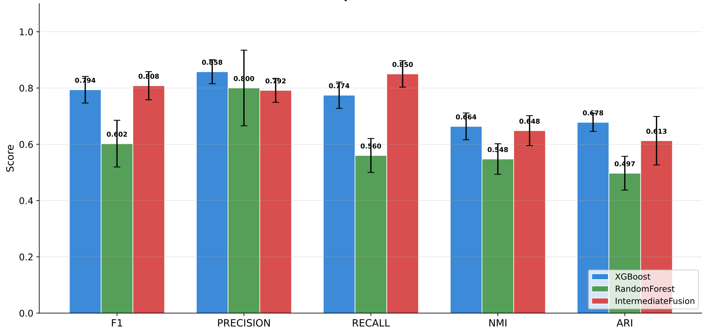
Model Comparison — GS-BRCA
