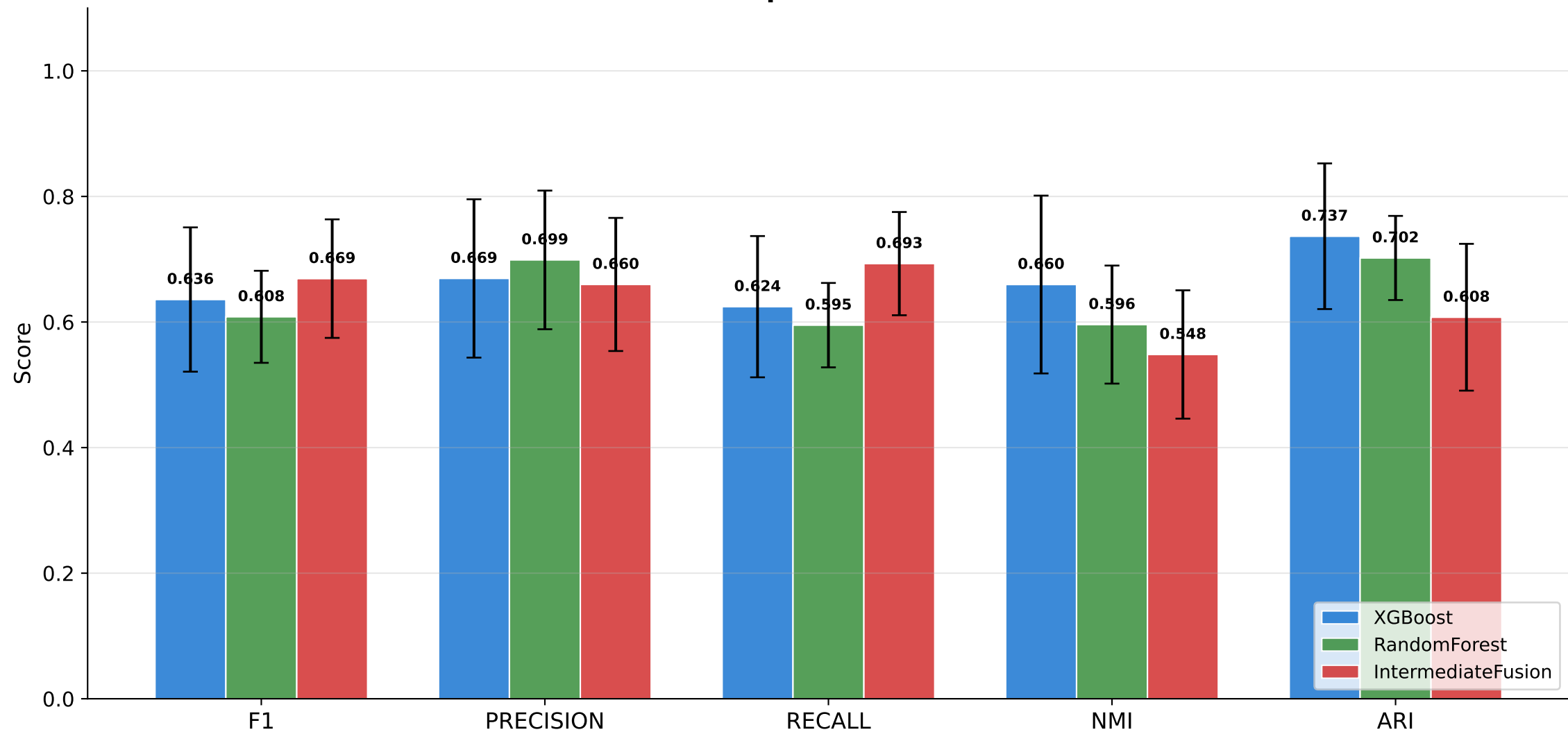
Model Comparison — GS-COAD
