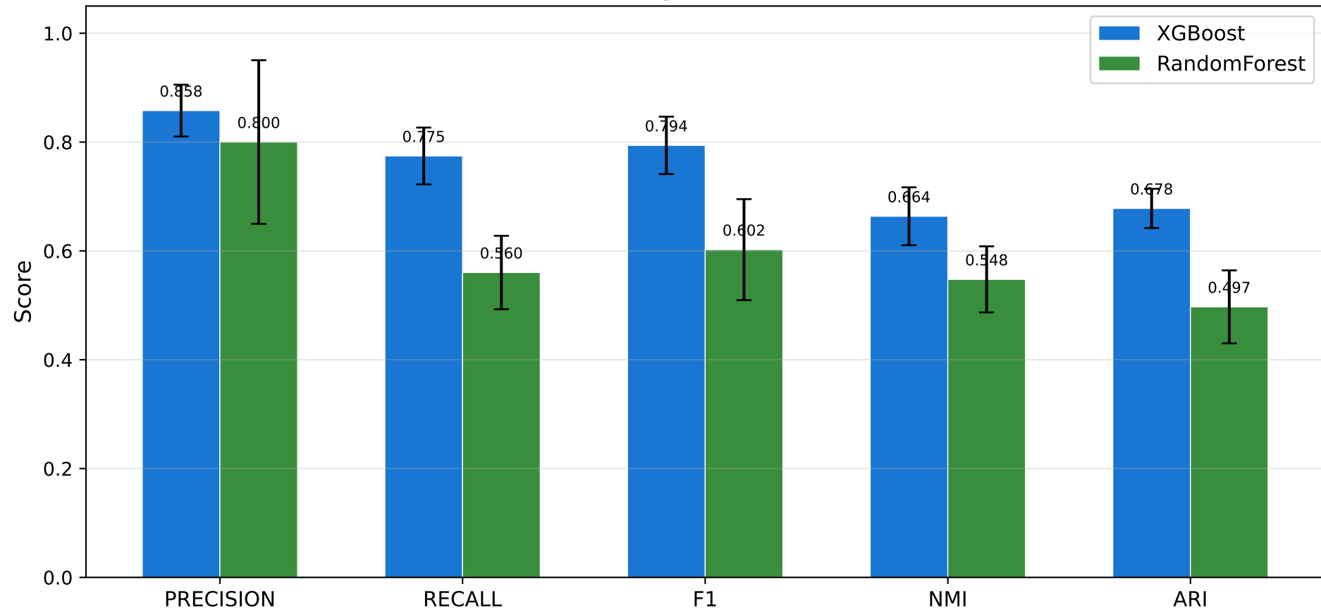
Baseline Comparison — GS-BRCA
