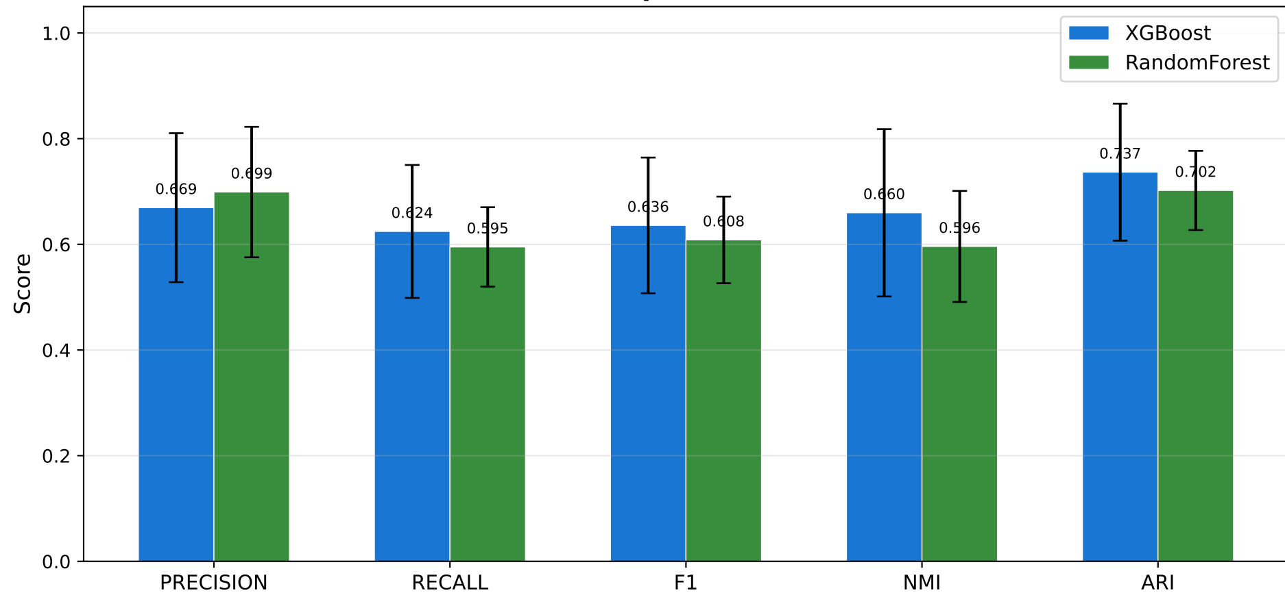
Baseline Comparison — GS-COAD
