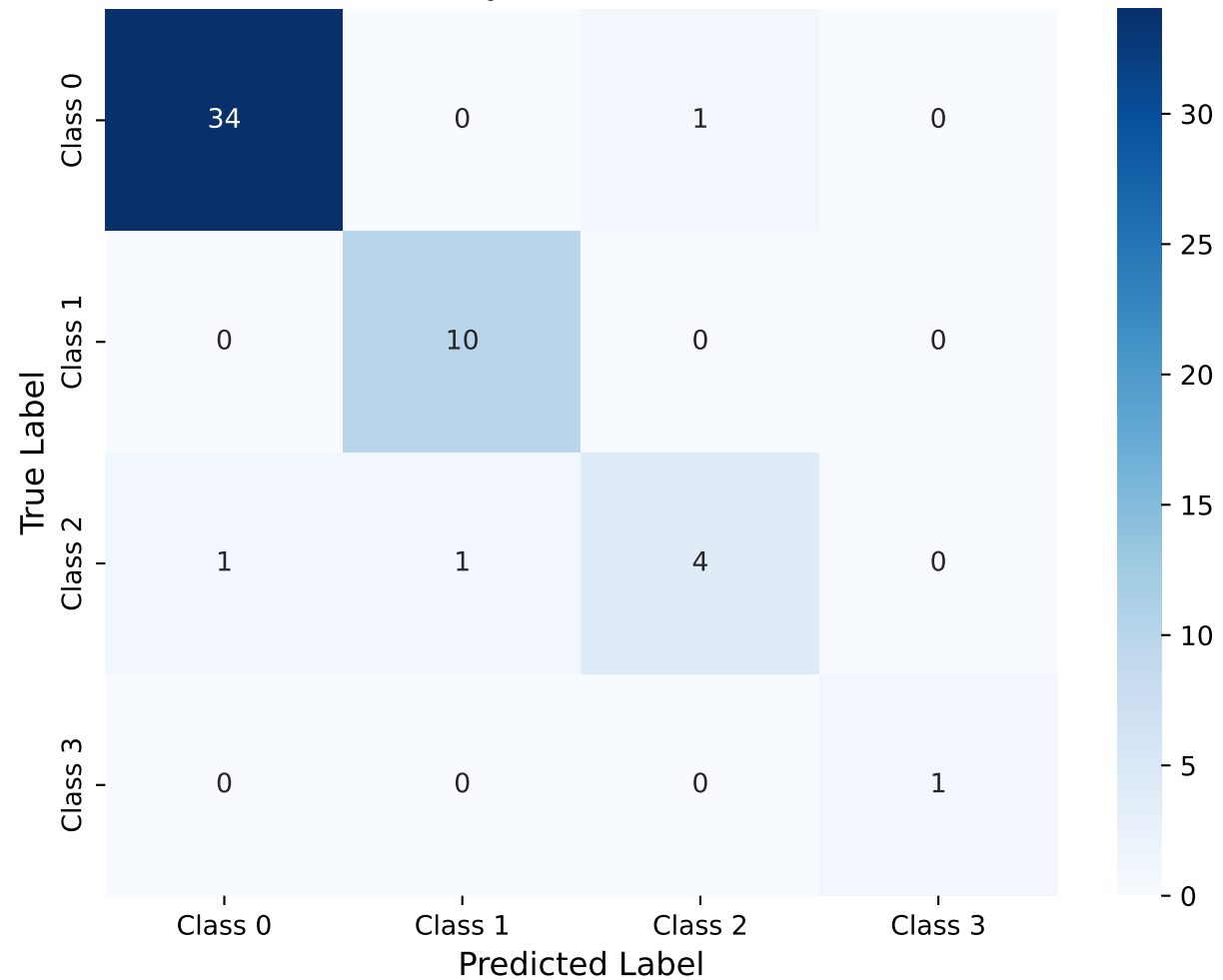
Confusion Matrix: PathwayAwareFusion (GS-COAD) - Best Fold
