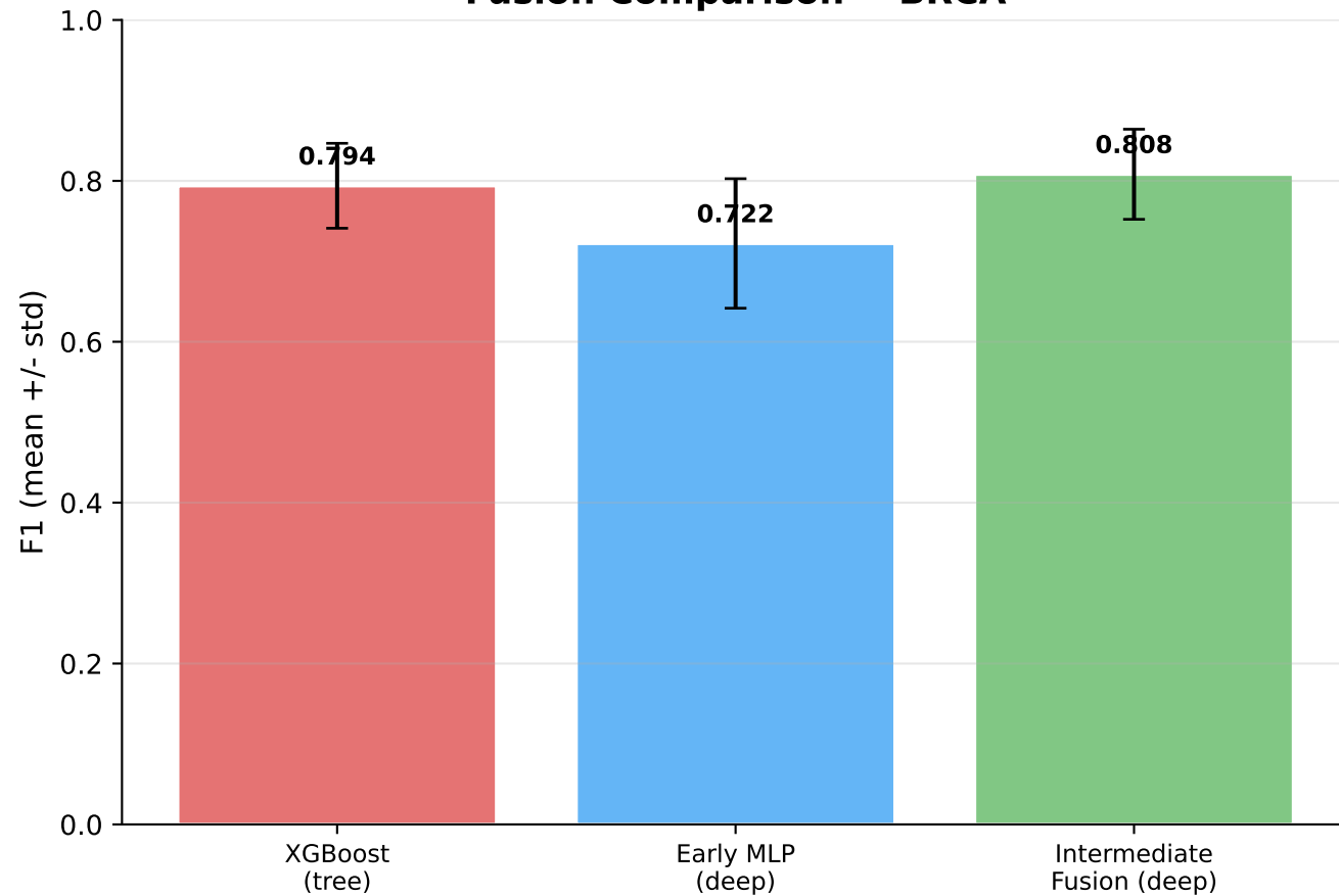
Fusion Comparison -- BRCA
