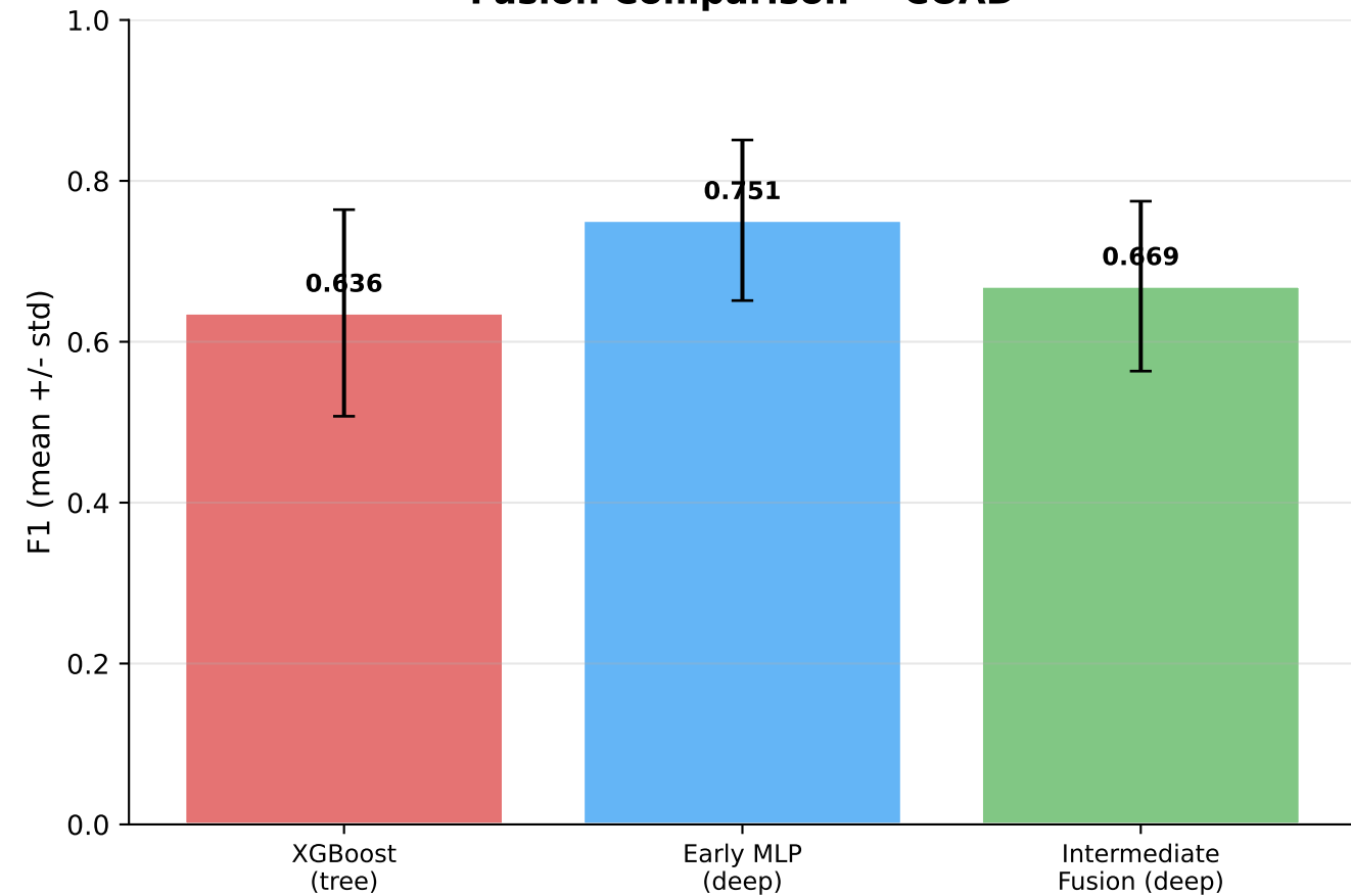
Fusion Comparison -- COAD
