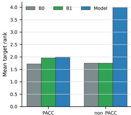
D. Rank by mutation class
