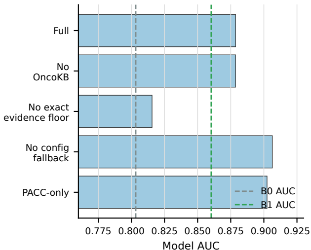
C. Design ablation
