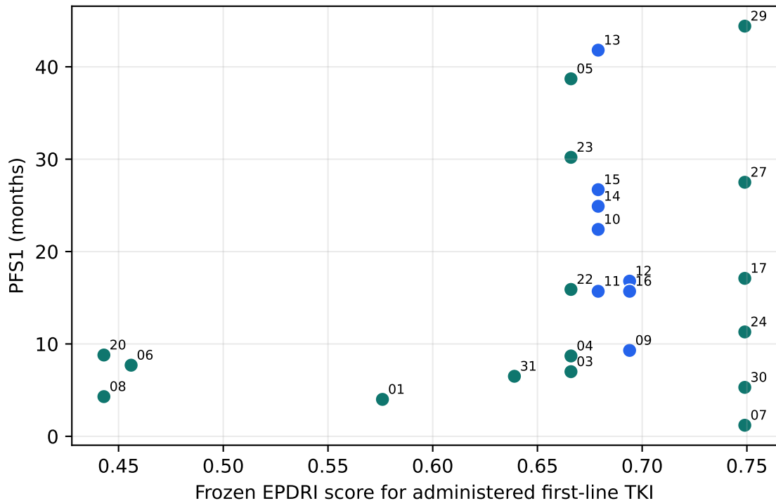
Local clinical validation: score vs PFS1
