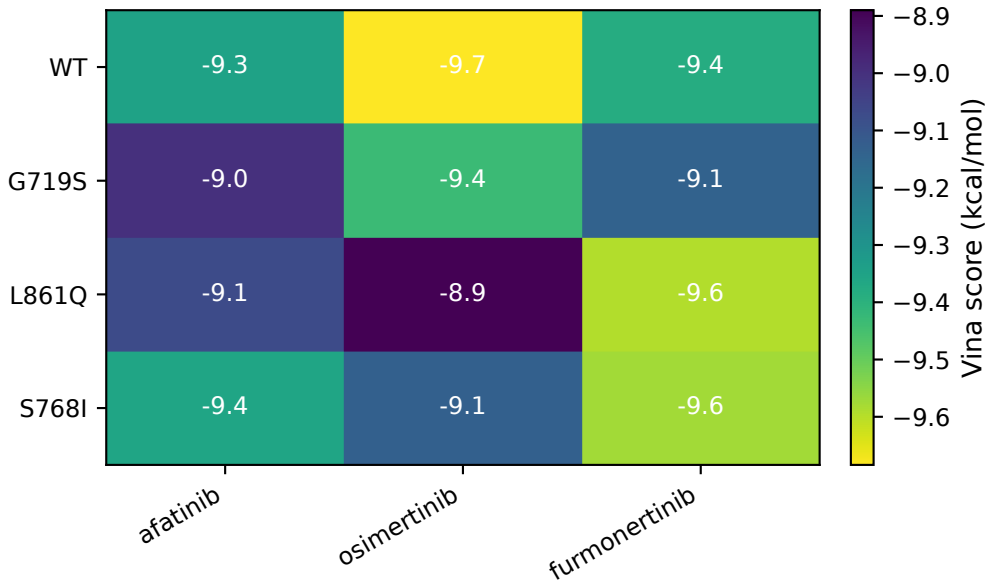
Basic Vina docking score matrix
