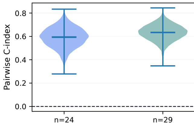
Pairwise C-index bootstrap violin
