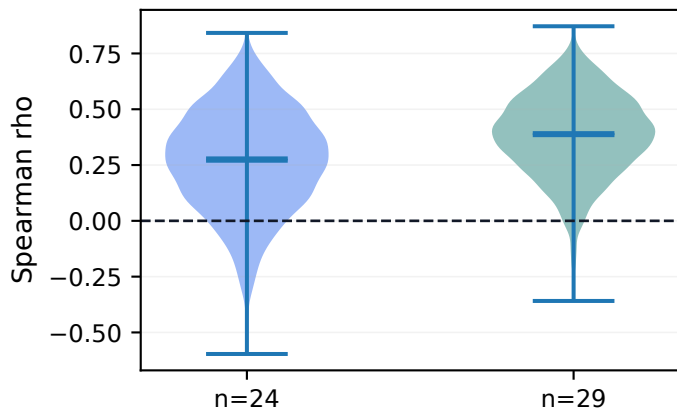
Spearman rho bootstrap violin
