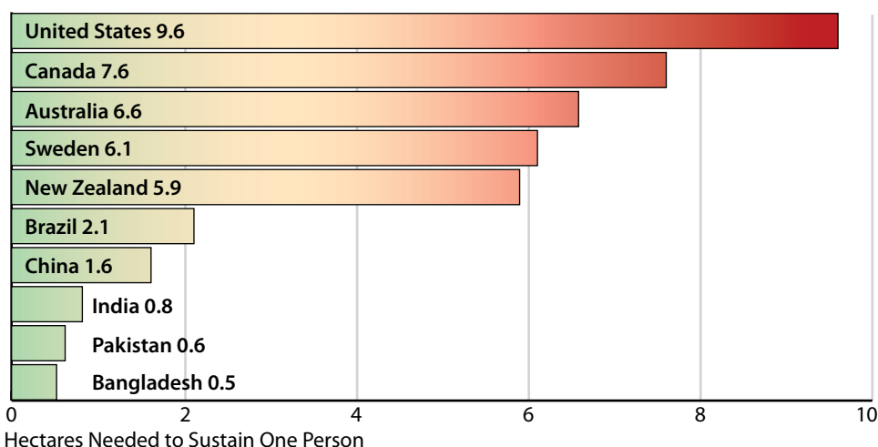
Figure 12-12 Ecological Footprints of Selected Countries, 2003
