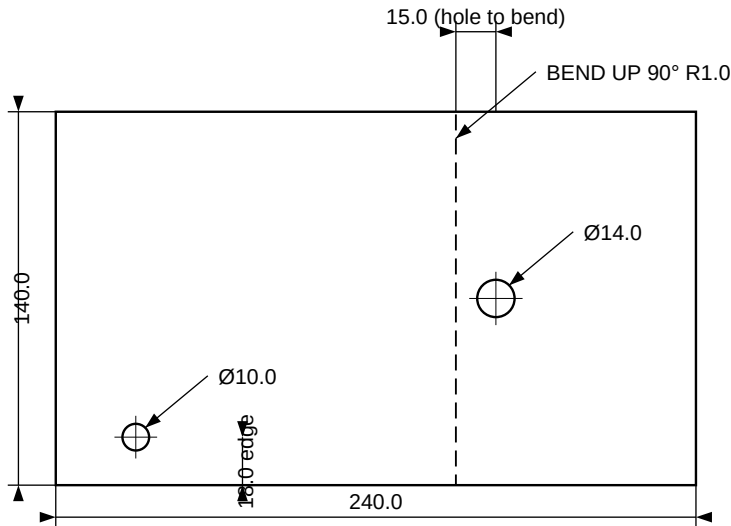
FLAT PATTERN
